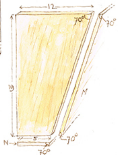
detail L
